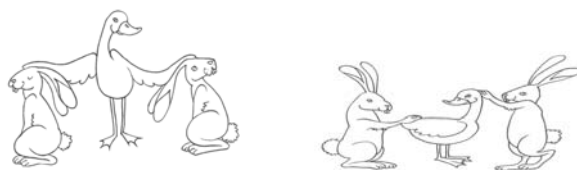
Fig. 4. A picture-pair used in task 2.
