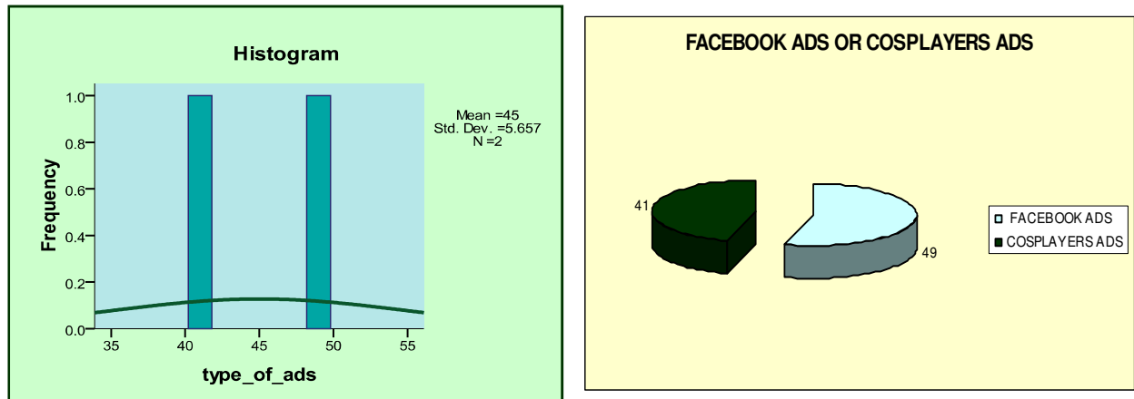
Figure no. 2 a) The frequencies histogram; b) The absolute frequencies pie graphical representation
