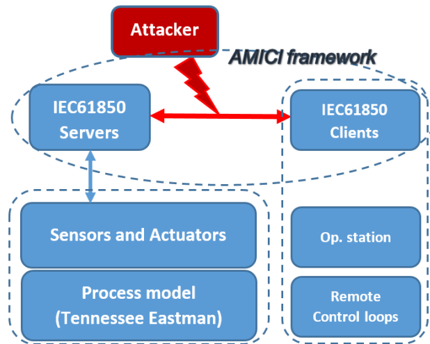
Fig. 2 AMICI extended with IEC 61850
