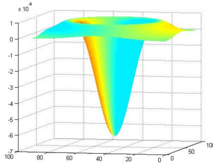
Figure 1 LoG operator
